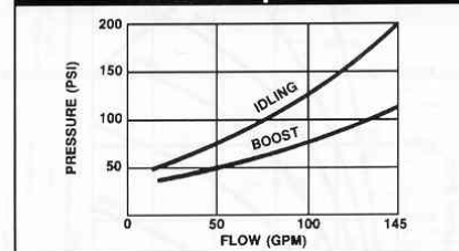
Idling Pressure and Boost Pressure Requirement
