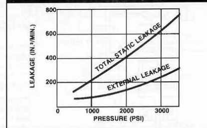
Static Leakage
