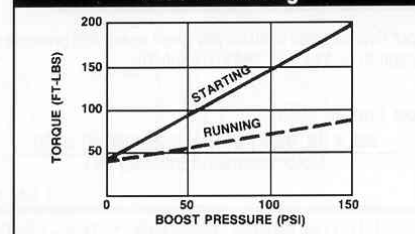
Torque Requirement When Free Wheeling
