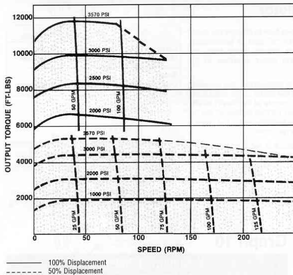
MRH2-270 Performance Curve
